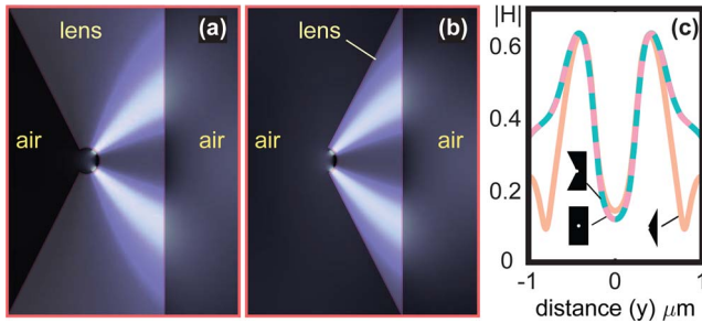
Fig. 3. (Color online) Open designs of the lens. (a) Magnetic field map inside a \frac{3}{4} -body lens. (b) Field map inside a \frac{1}{4} -body lens. Shaded areas indicate the lens cross-section in (a) and (b). (c) H-field generated by the sources along the flat surface of either the closed or open lens designs.
